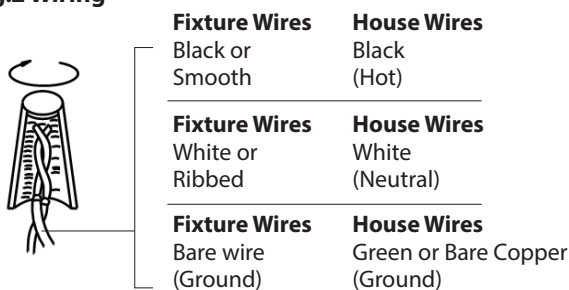
Fig.2 Wiring
